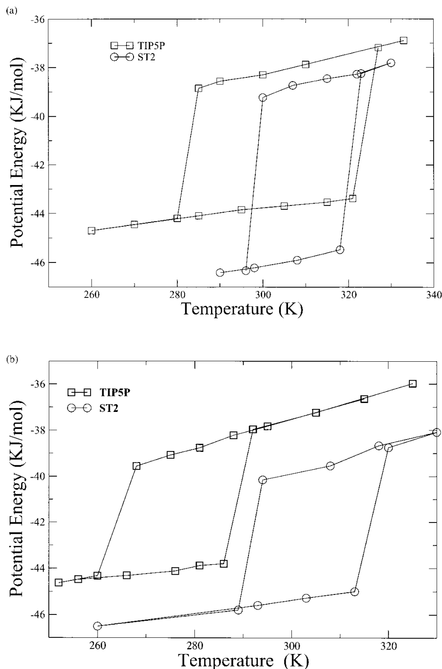
FIGURE 1 Temperature dependence of the QPE in (a) system I and (b) system II.
