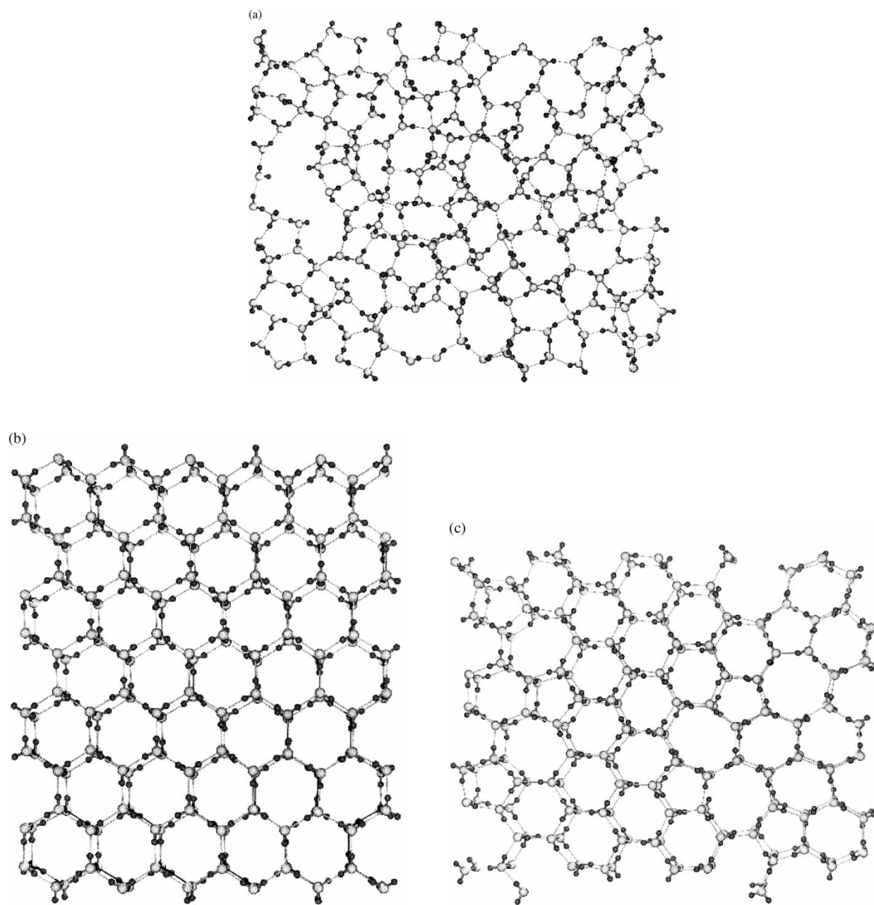
FIGURE 2 Quenched structures of the confined water in the state of (a) liquid, (b) bilayer crystal and (c) amorphous bilayer ice. Larger spheres denote oxygen and smaller spheres denote hydrogen.
