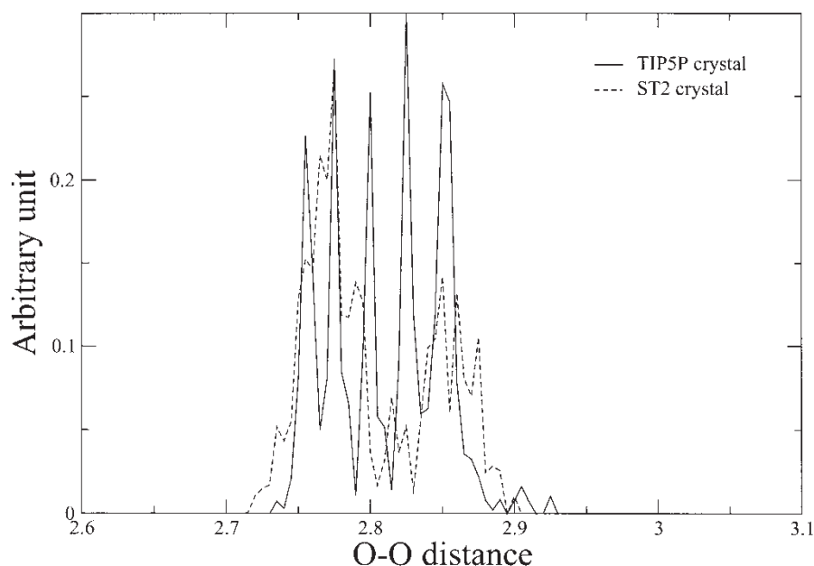
FIGURE 4 The O—O bond length distribution of TIP5P and ST2 bilayer crystals.
