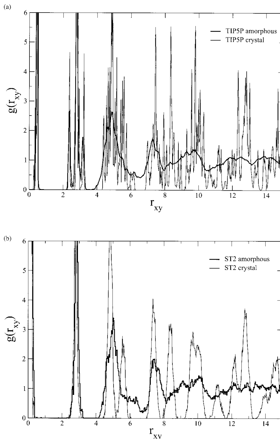
FIGURE 5 Two-dimensional radial distribution of oxygen of (a) TIP5P and (b) ST2 bilayer crystal and amorphous bilayer ice.
